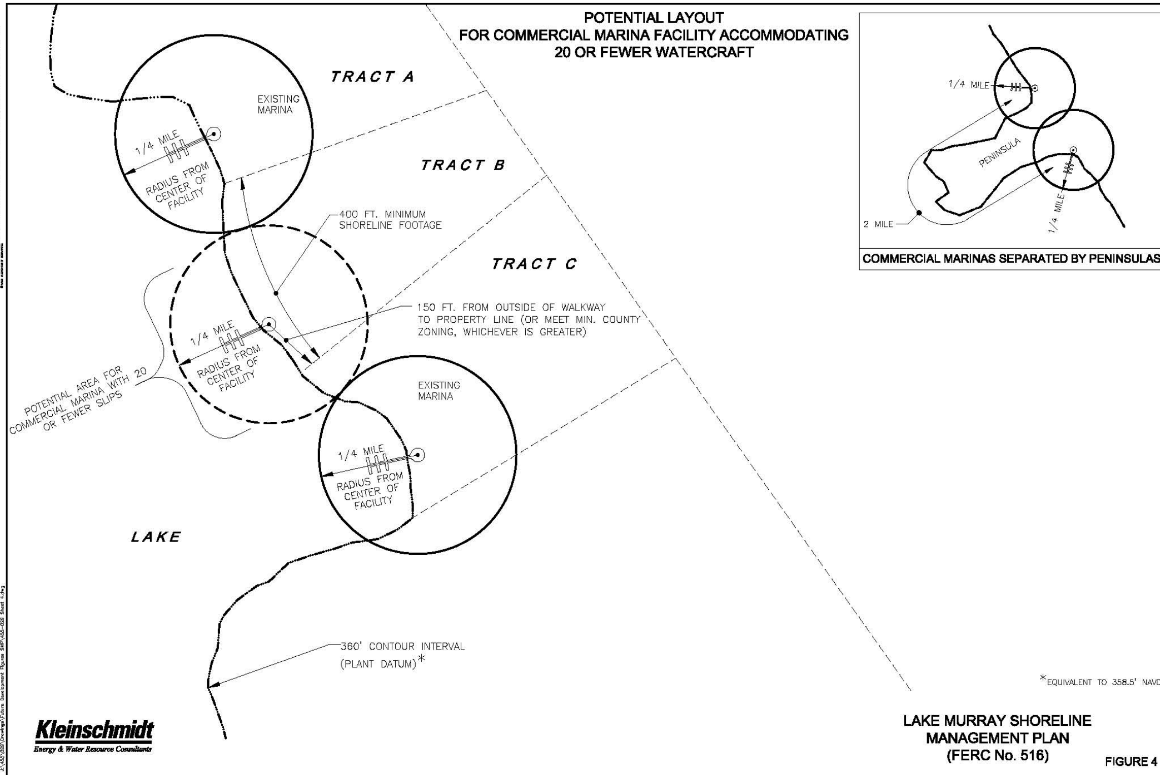
Figure 9.3-8: Potential Layout for Commercial Marina Facility Accommodating 20 or Fewer Watercraft
