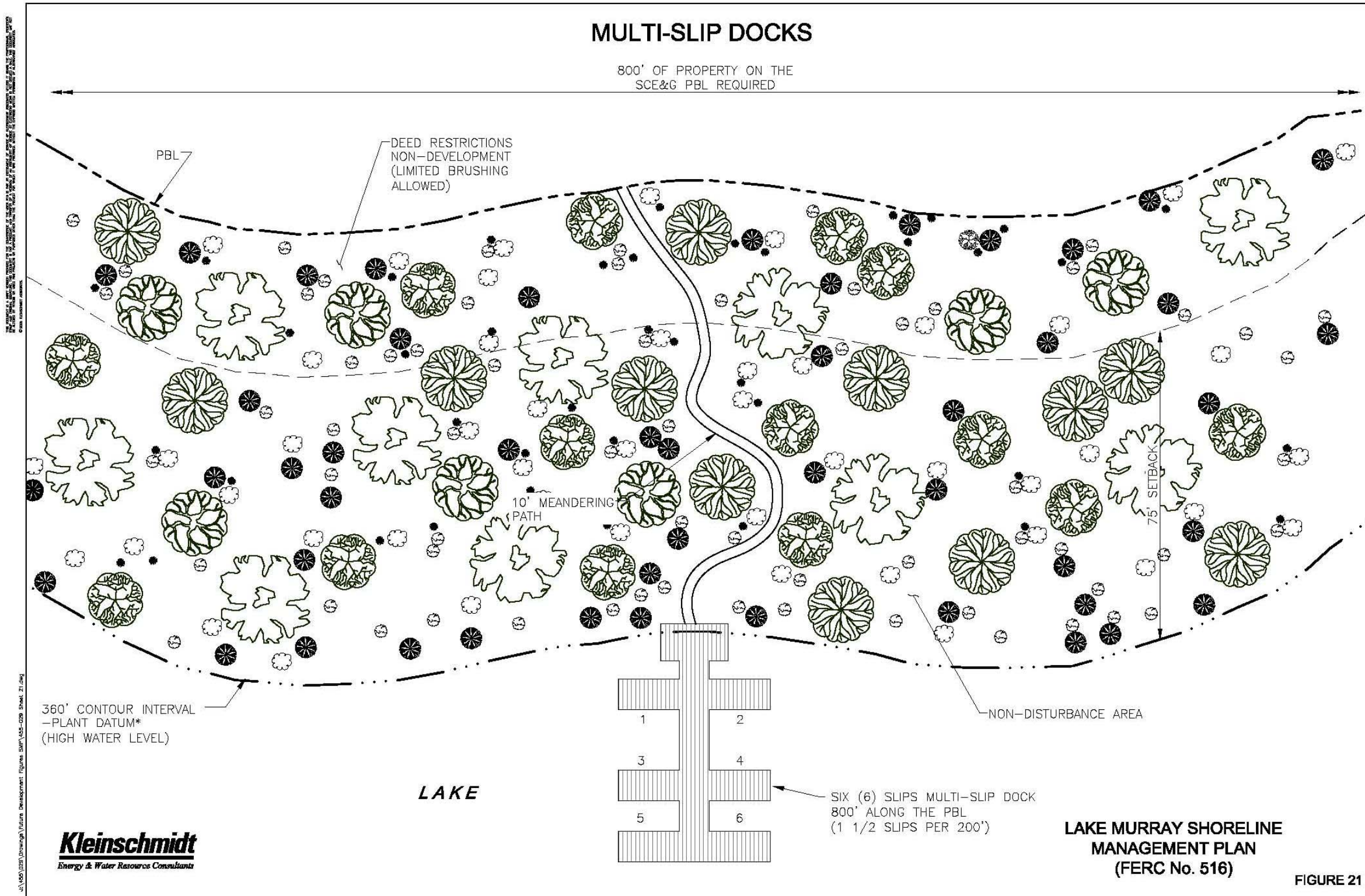
Figure 7.2-7: Example of Multi-slip Dock Layout
